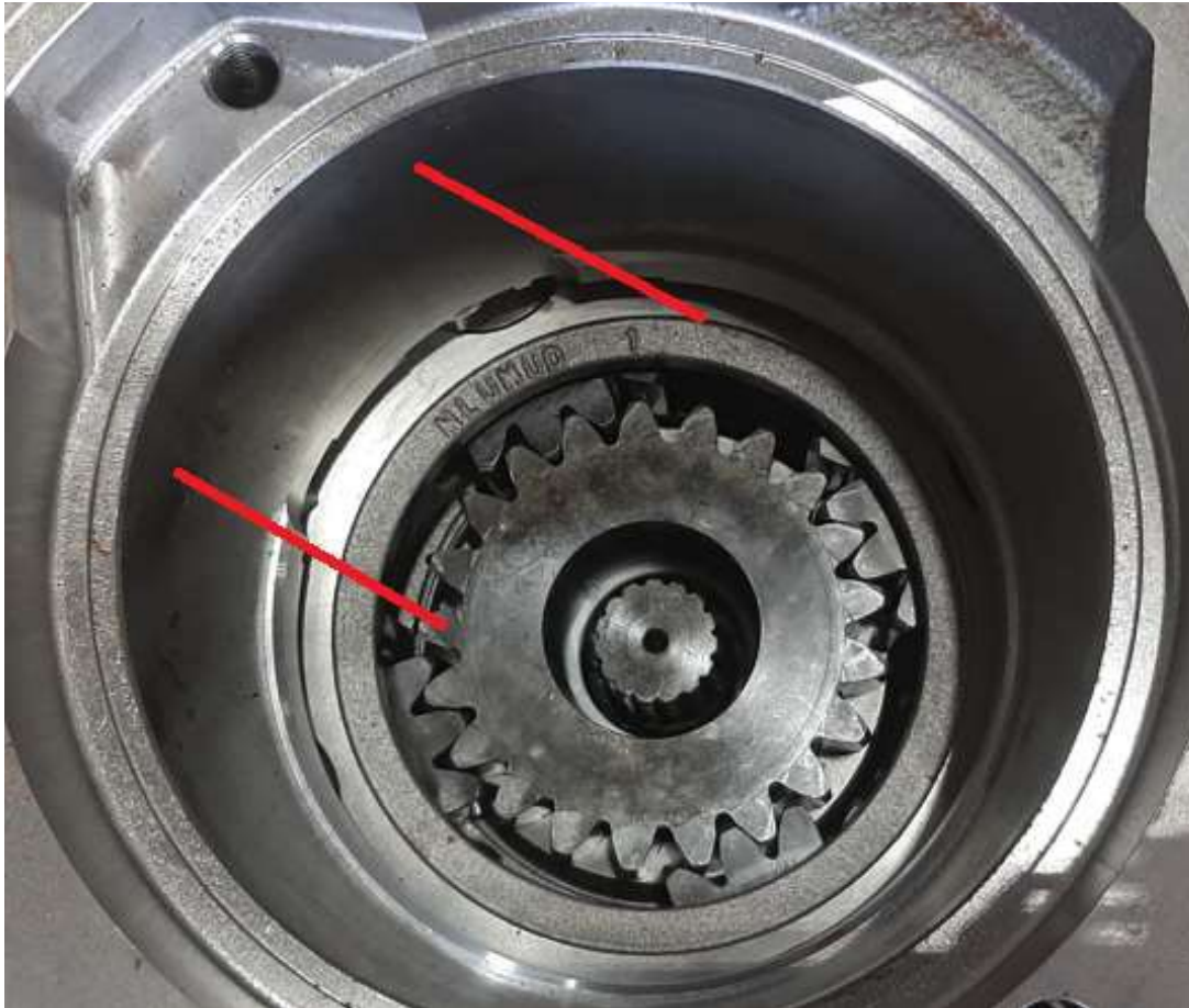
Image 1 – Gear-Coupling mistaken assembly.
